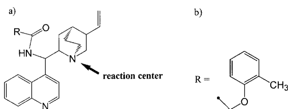
Figure 2. The chiral base that yielded the highest ee out of the 30 bases screened [12]
